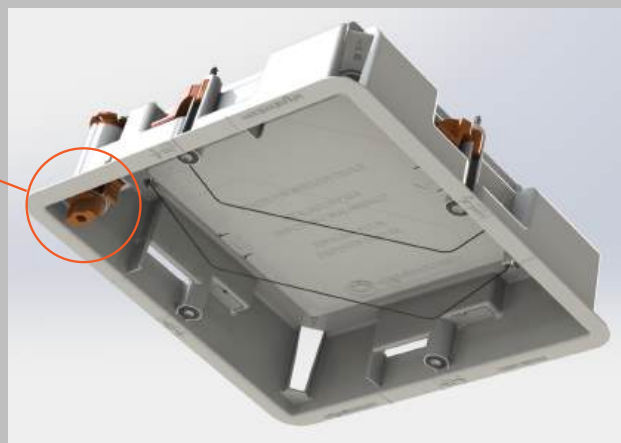
Ratcheting lock system for easy installation.
